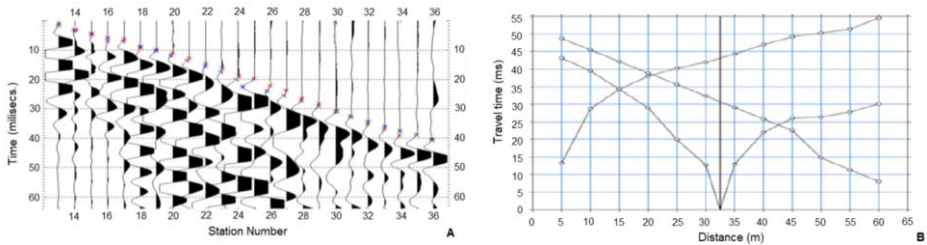
Figure 6. A. Record of arrival times of seismic waves to sensors; B. Dromochrones of the seismic line.
