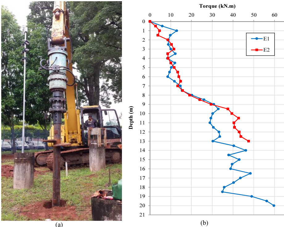
Figure 5. (a) Pile installation and (b) results of installation torque.
