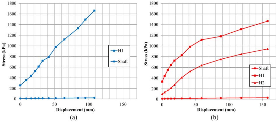
Figure 9. Helix bearing pressure and shaft skin friction during the loading tests on piles E1 and E2.
