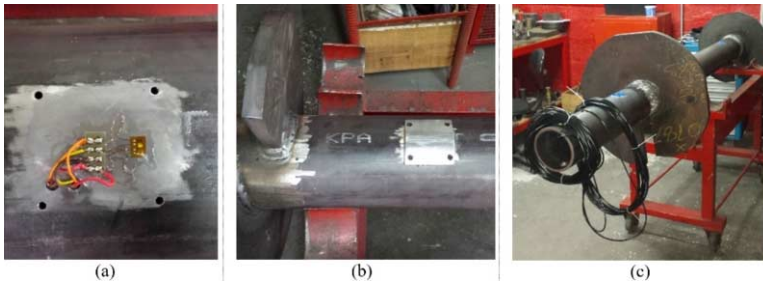
Figure 4. Details of pile instrumentation: (a) strain gages, (b) mechanical protection of sensors, and (c) cables connected to the strain-gages (cables passing through the shaft).
