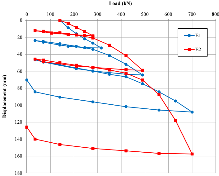
Figure 7. Applied load at pile head versus displacement for axial tension pile load tests.
