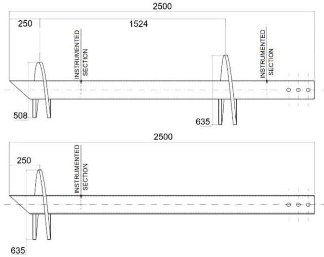
Figure 3. Dimensions of the lead sections of the tested piles E1 and E2 (millimeters).
