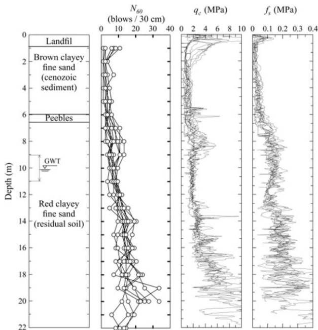
Figure 2. Soil profile at the test site ([8]).
