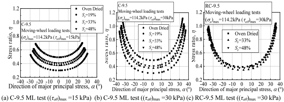
Figure 5. Stress paths analyzed.
