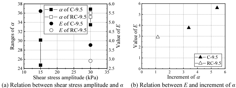
Figure 6. Synergistic effect of principal stress axis rotation and change in moisture content.
