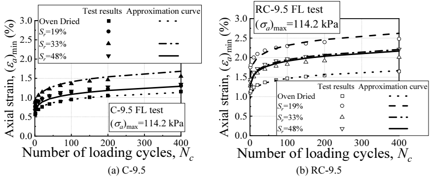
Figure 3. Estimation of the permanent axial strain in FL tests.
