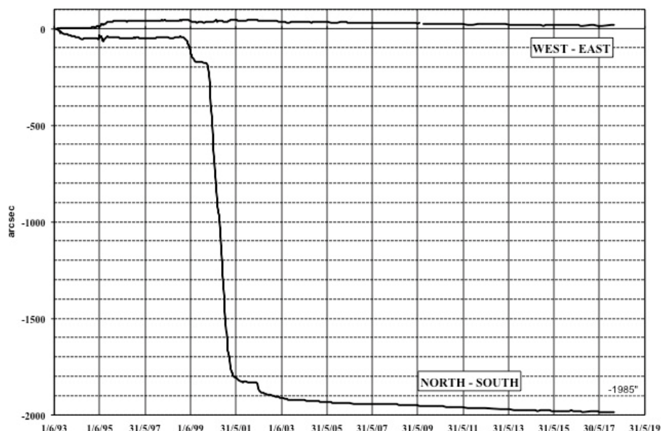
Figure 7. Rotation of the foundation of the Tower since 1993.
