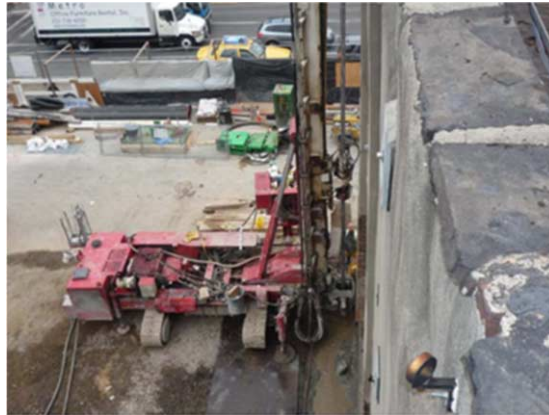
Figure 5. Jet grouting adjacent to existing building.
