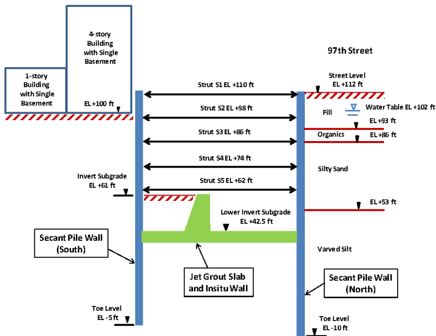
Figure 2. Excavation support system for construction of Ancillary 2.
