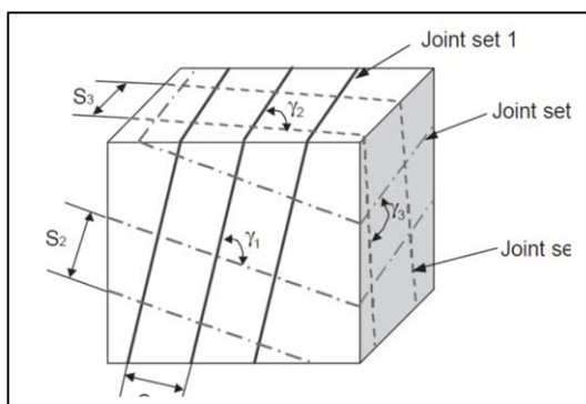
Figure 1. Rock mass with three joint sets –after Palmstrom [14].
