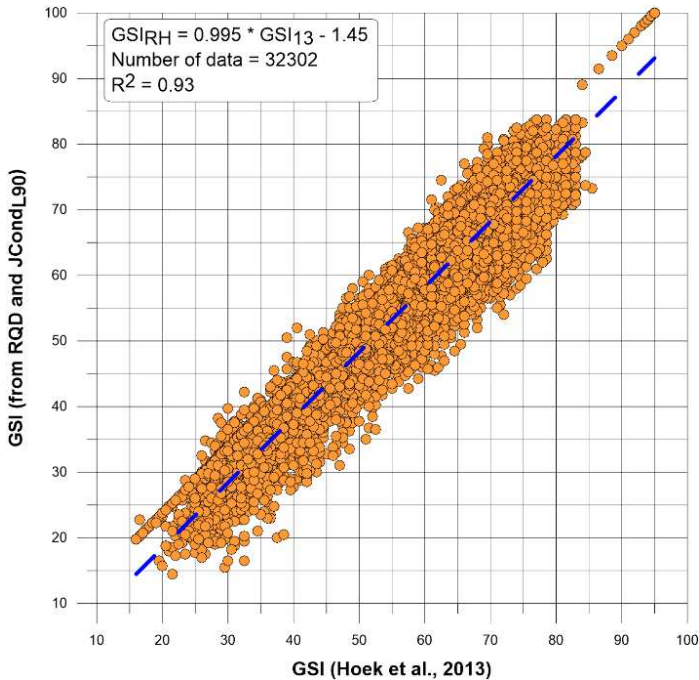
Figure 7. Correlation graph between GSI estimated from RQD and joint condition JCond 90 from Laubscher and GSI from Hoek et al. [15].
