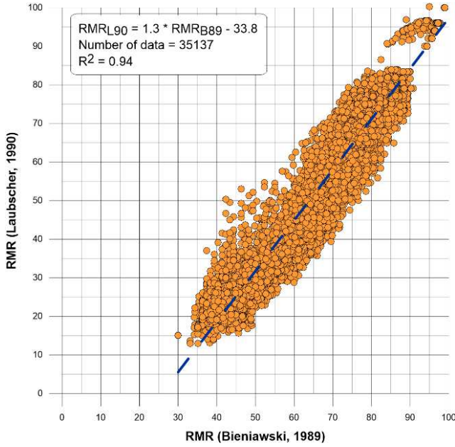
Figure 4. Laubscher RMR [1] vs. Bieniawski RMR [2] correlation.
