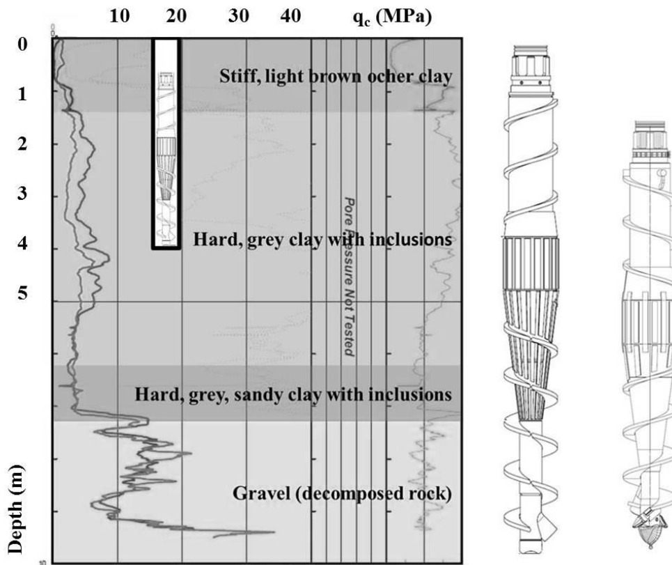
Figure 1. Typical soil profile at Lawnton test site (left), rapid displacement auger used for test piles D and E (centre), and progressive displacement auger used for test pile C
