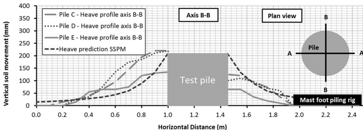
Figure 4. Schematic soil heave profiles for test piles C, D & E and SSPM prediction (axis B-B)
