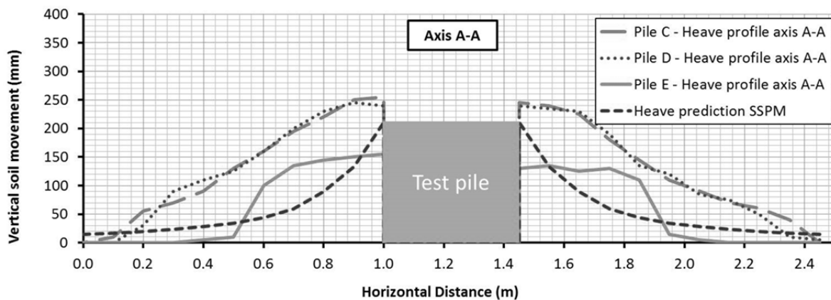
Figure 3. Schematic soil heave profiles for test piles C, D & E and SSPM prediction (axis A-A)
