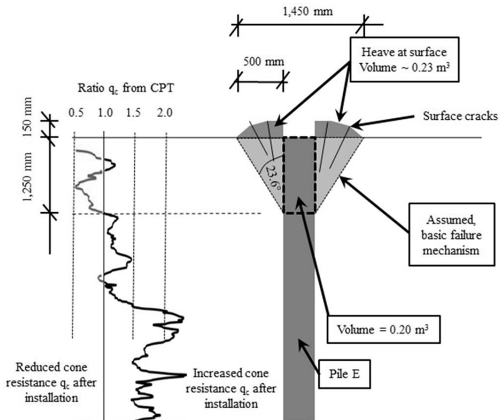
Figure 7. Schematic heave cone, heave volume and CPT ratio for test pile E (not to scale)
