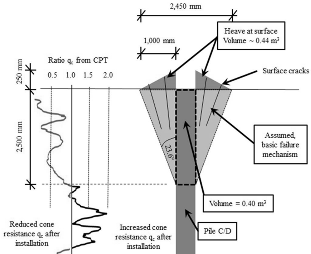
Figure 6. Schematic heave cone, heave volume and CPT ratio for test piles C and D (not to scale)
