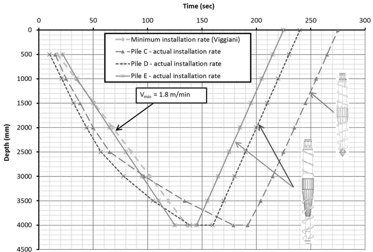
Figure 2. Installation and extraction rates of test piles C, D and E
