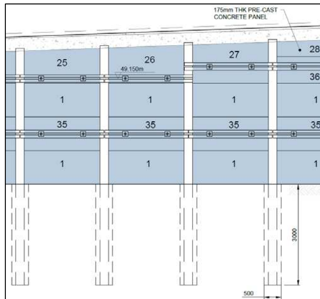
Figure 2. Design elevation for Cunningham Terrace retaining wall
