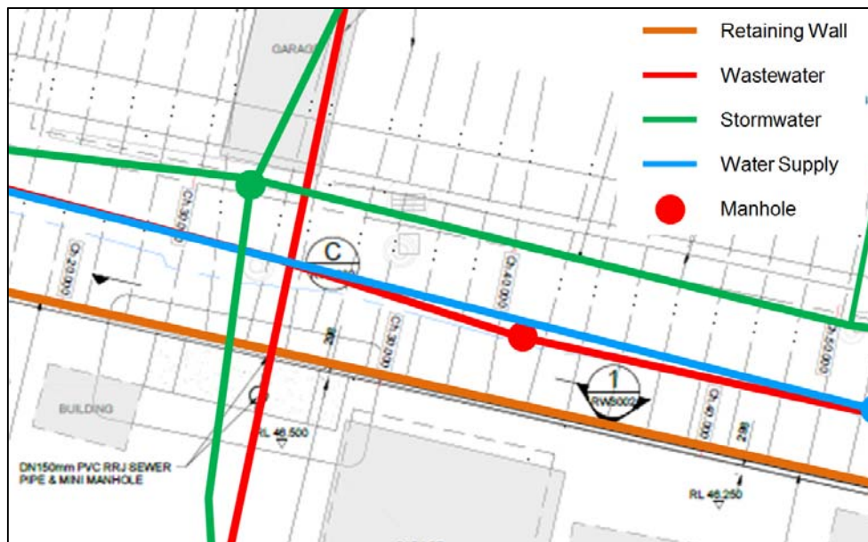
Figure 5. Buried Services adjacent to Cunningham Terrace Retaining Wall
