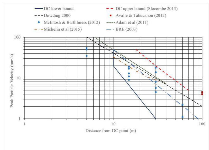
Figure 5. DC vibration decay.
