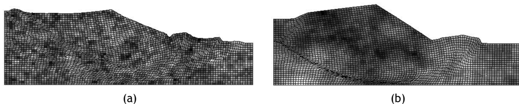
Figure 2: Typical random field realisations with scale of fluctuation of (a) 1 m and (b) 10 m.
