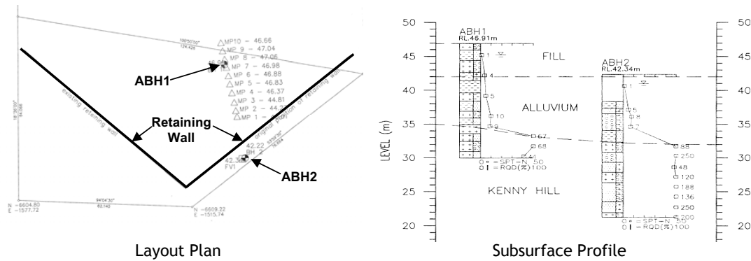
Figure 3: Additional SI Layout Plan and Profile
