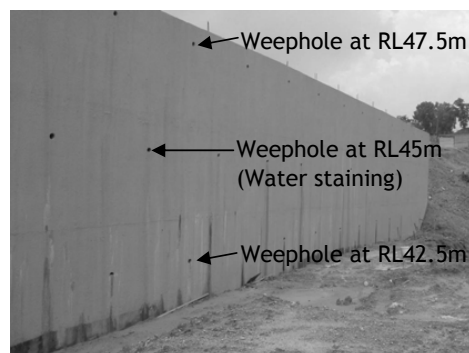
Figure 1: Overall Site Conditions and Water Staining at Weephole Drains
