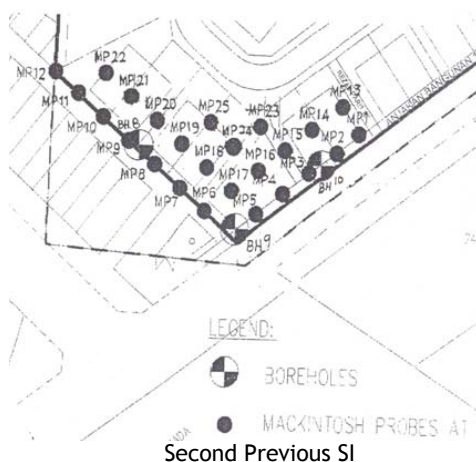
Figure 2: Previous SI Layout Plan
