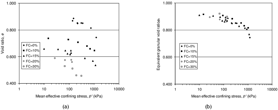
Figure 2: (a) Multiple SSLs for sand with fine, (b) Equivalent granular SSL for sand with fines
