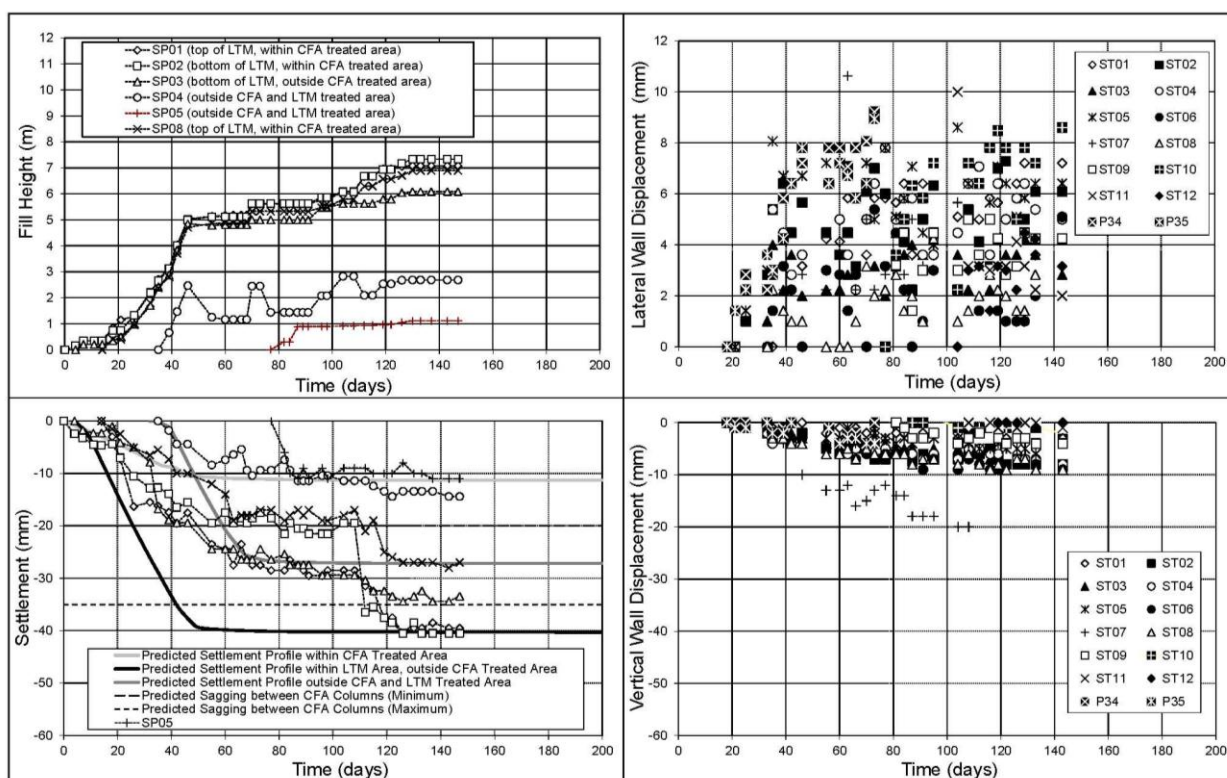
Figure 7. Settlement and lateral movement monitoring
