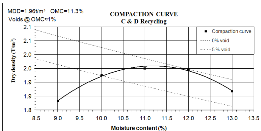
Figure 1: The C & D Recycling compaction curve.
