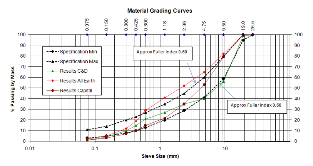
Figure 4: Particle size distributions for recycled materials.
