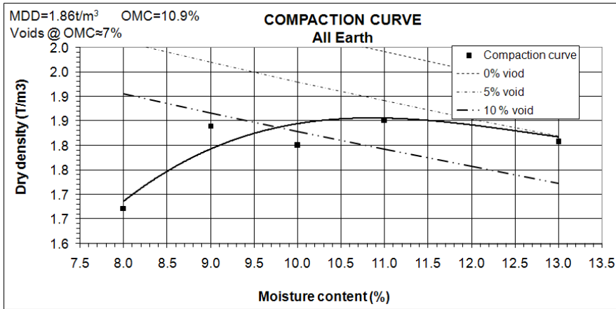
Figure 2: The all Earth compaction curve.
