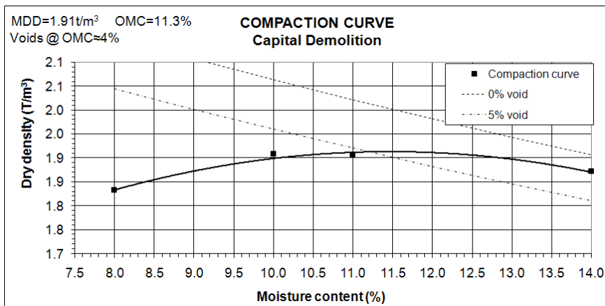
Figure 3: The Capital Demolition compaction curve.
