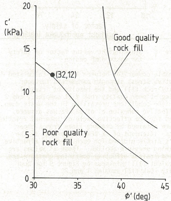
Figure 7 Back-calculated effective stress strength parameters
