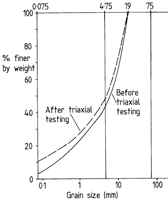
Figure 3 Particle size distribution curves for before and after triaxial testing of sample 1
