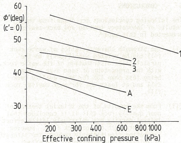
Figure 5 \phi' versus effective confining pressure for Bougainville rock fill
