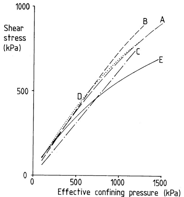
Figure 2 Comparison of failure envelopes
