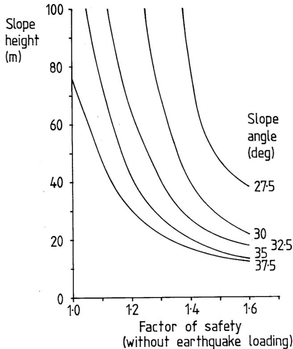
Figure 8 Slope height versus factor of safety for waste dump design
