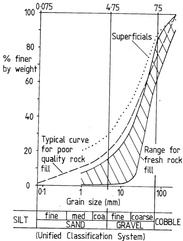
Figure 1 Particle size distribution curves
