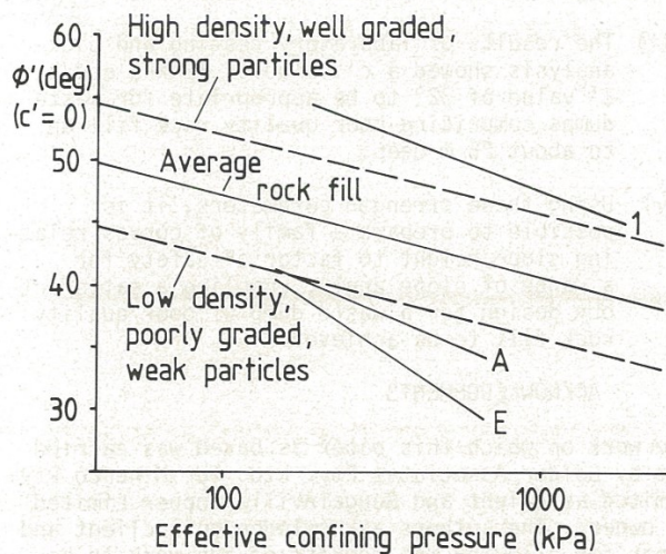
Figure 6 \phi' versus effective confining pressure for other rock fill
