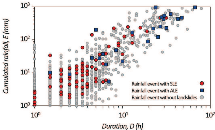
Figure 3. Rainfall duration ( D ) vs. cumulated rainfall ( E ) in Emilia-Romagna from March 2014 to December 2015. Red circles are 78 ED rainfall conditions associated with the triggering of SLEs. Blue squares are the 24 ED rainfall conditions associated with the triggering of ALEs. Grey circles are 927 rainfall events representative of non-triggering rainfall conditions. Data are in log-log coordinates.
